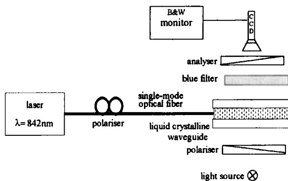
FIGURE 3 Experimental setup
