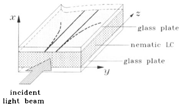
FIGURE 1 Schematic drawing of the analysed waveguide configuration. For low powers the light beam diffracts in zy plane (dashed lines) but for high powers it can be self-trapped (solid lines).
