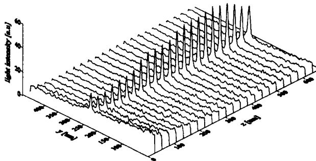
FIGURE 4 Scattered light intensity measured for the input power (A) P < 20\text{mW} , (B) P \approx 20\text{mW} and TE-like polarized input, and (C) P \approx 30\text{mW} and TM-like polarization.
